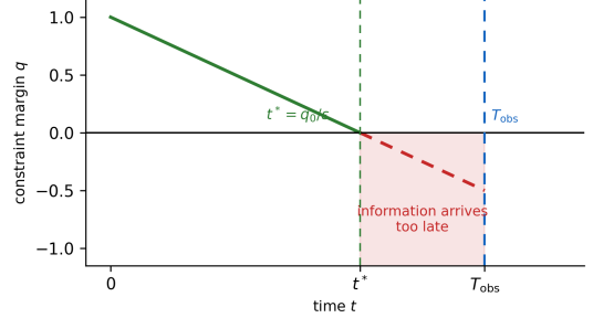
Figure 2: Delayed information. The constraint margin q reaches zero at t^* = q_0/\epsilon , before the first informative observation at T_{\text{obs}} : the information is accurate but arrives too late (Theorem 3).
